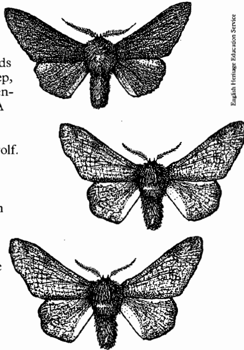
Peppered moths are camouflaged to merge in to the background.
