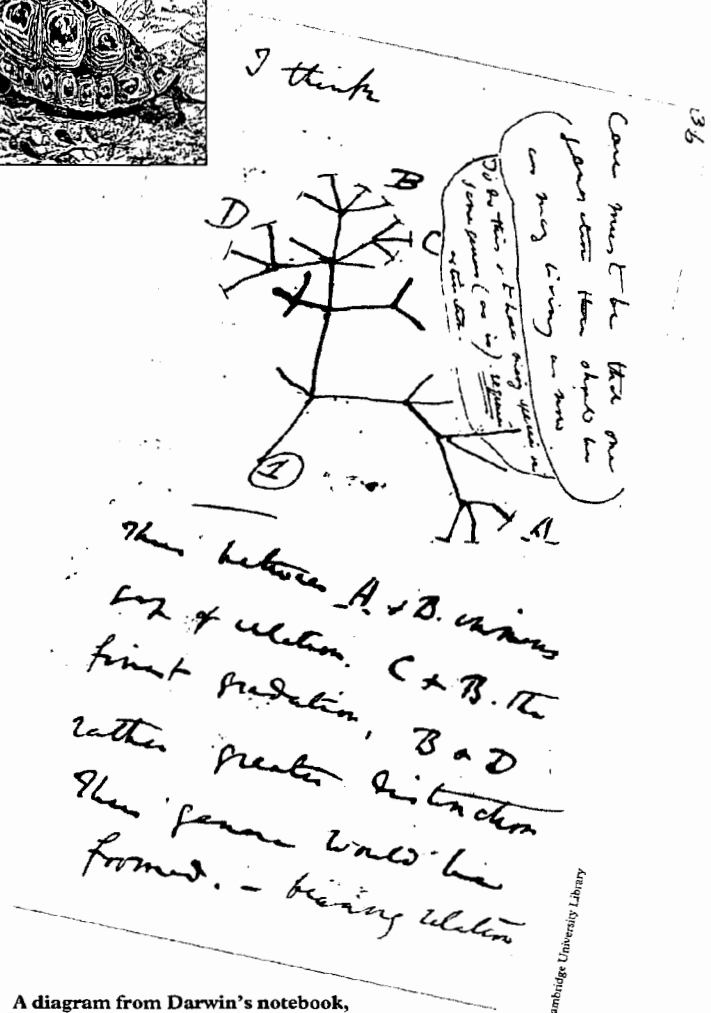
A diagram from Darwin's notebook, to illustrate branching evolution.
