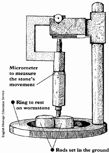
Darwin devised a special instrument to help him measure the action of worms in the soil. He placed a millstone on his lawn, with this instrument placed in the middle, to measure how far the stone sank each year.
