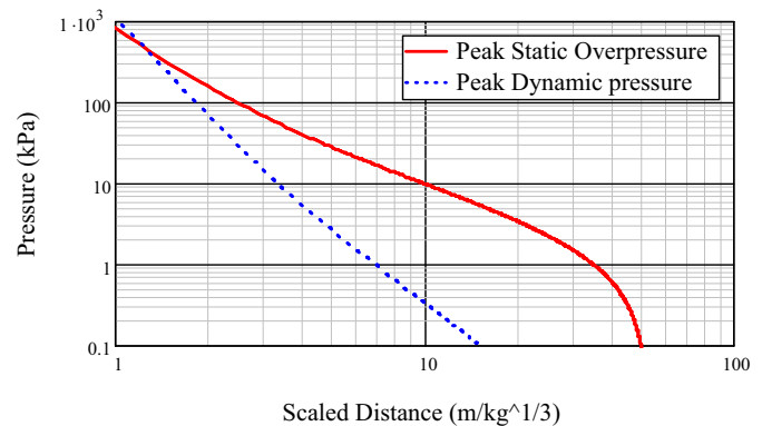
Figure 3. Traces of peak static and dynamic pressures vs. scaled distance (closed form solution)[17]
