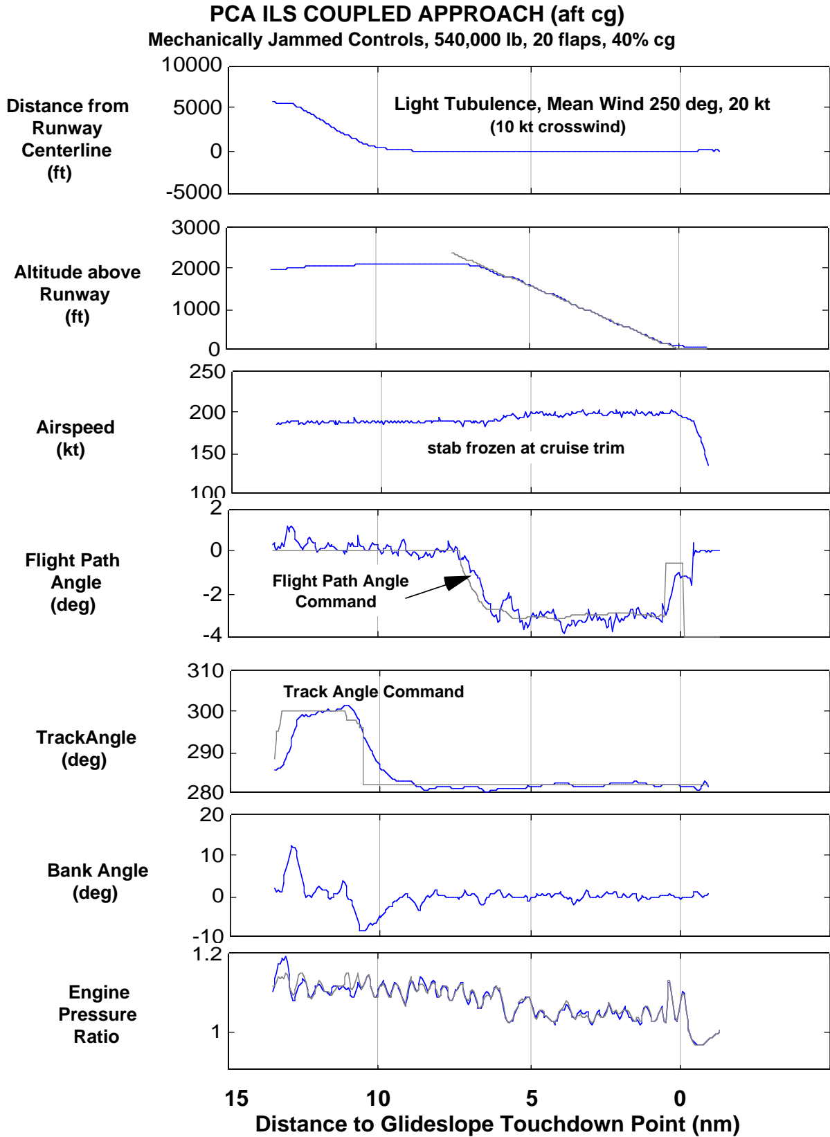
Figure 17. PCA fully coupled approach with aft center of gravity.
