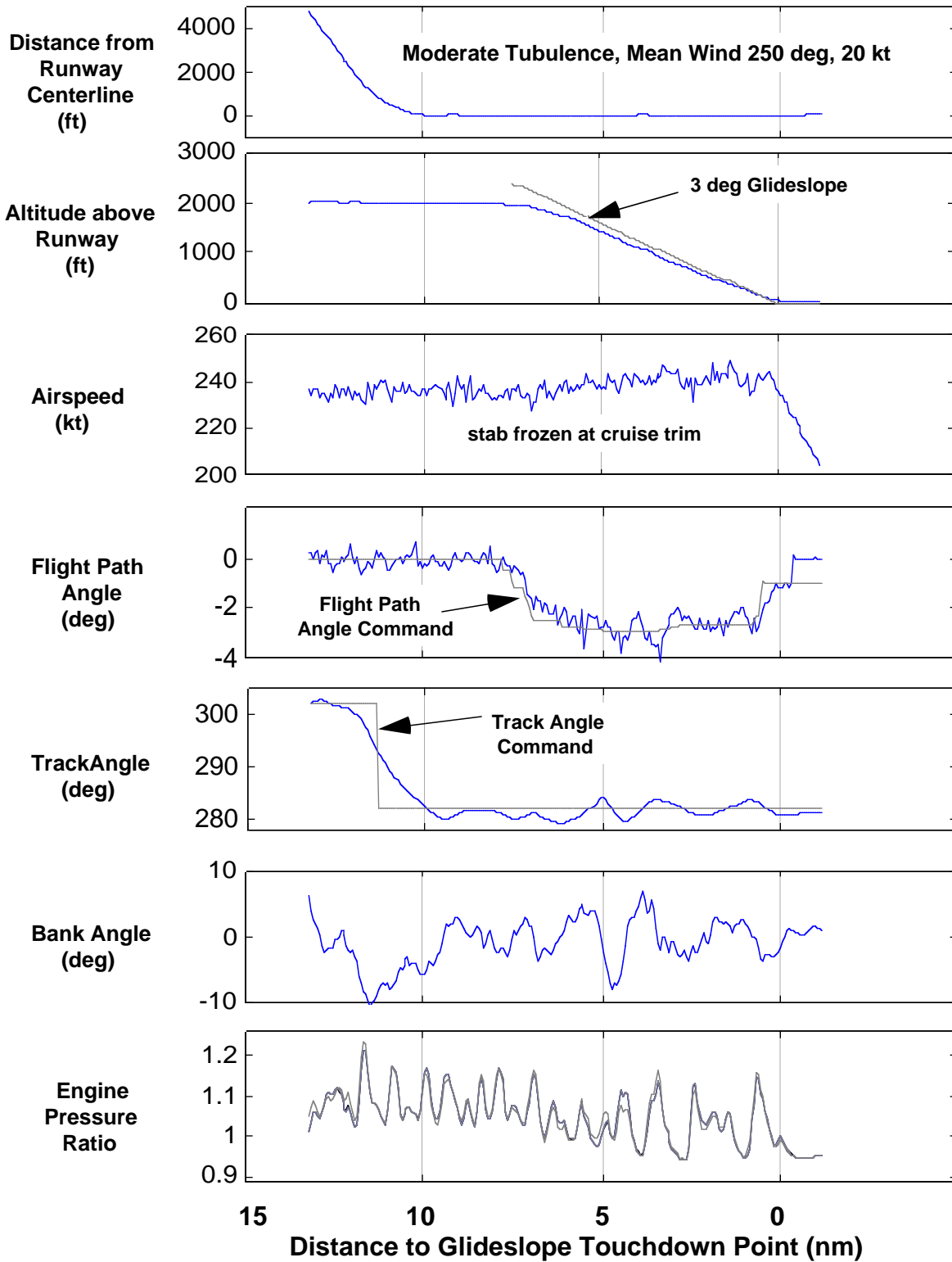
Figure 16. PCA localizer only coupled approach with moderate turbulence.
