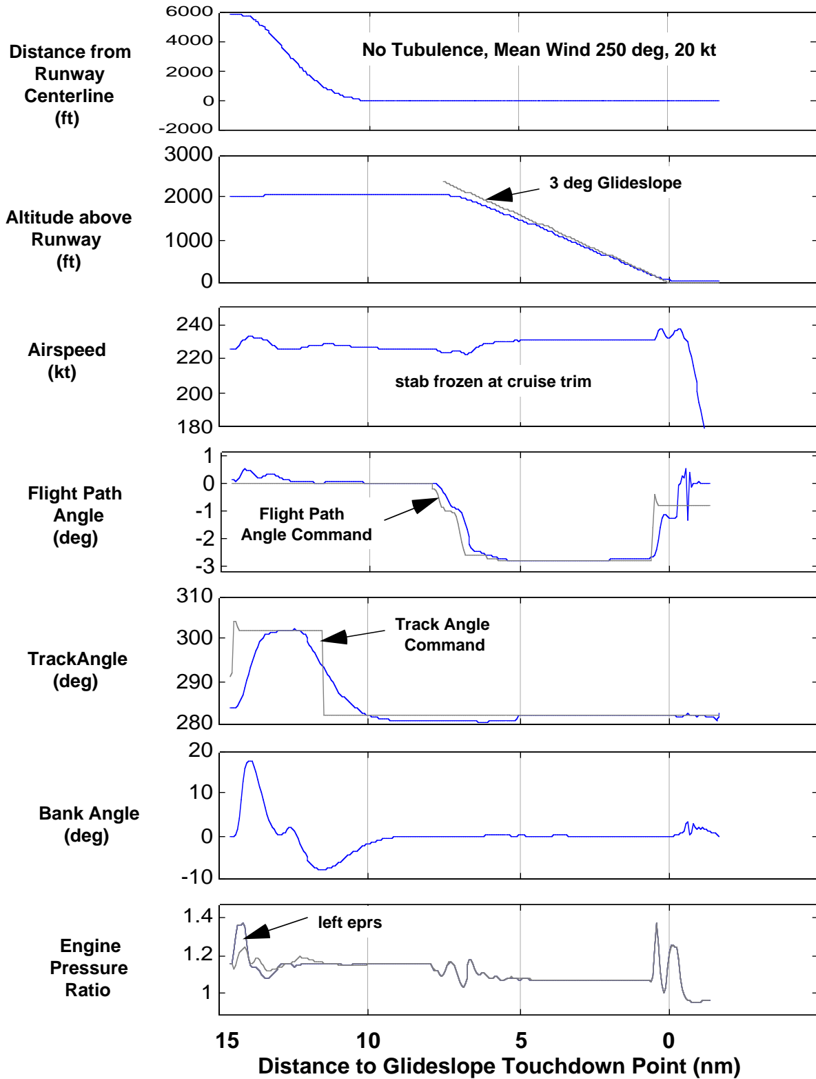
Figure 15. PCA localizer only coupled approach with no turbulence.
