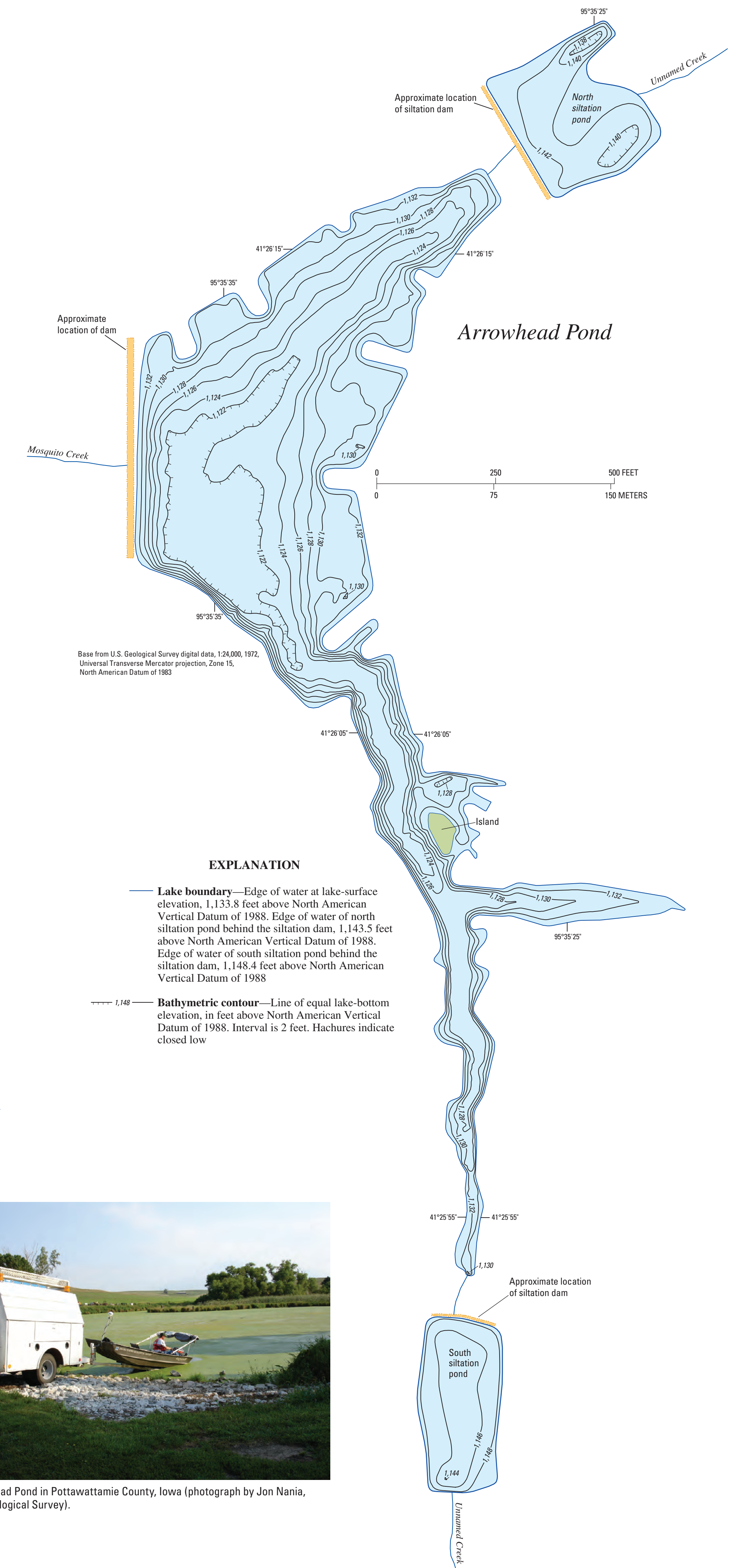
Figure 2. Bathymetric contours of Arrowhead Pond, 2005 (not for navigational use).
