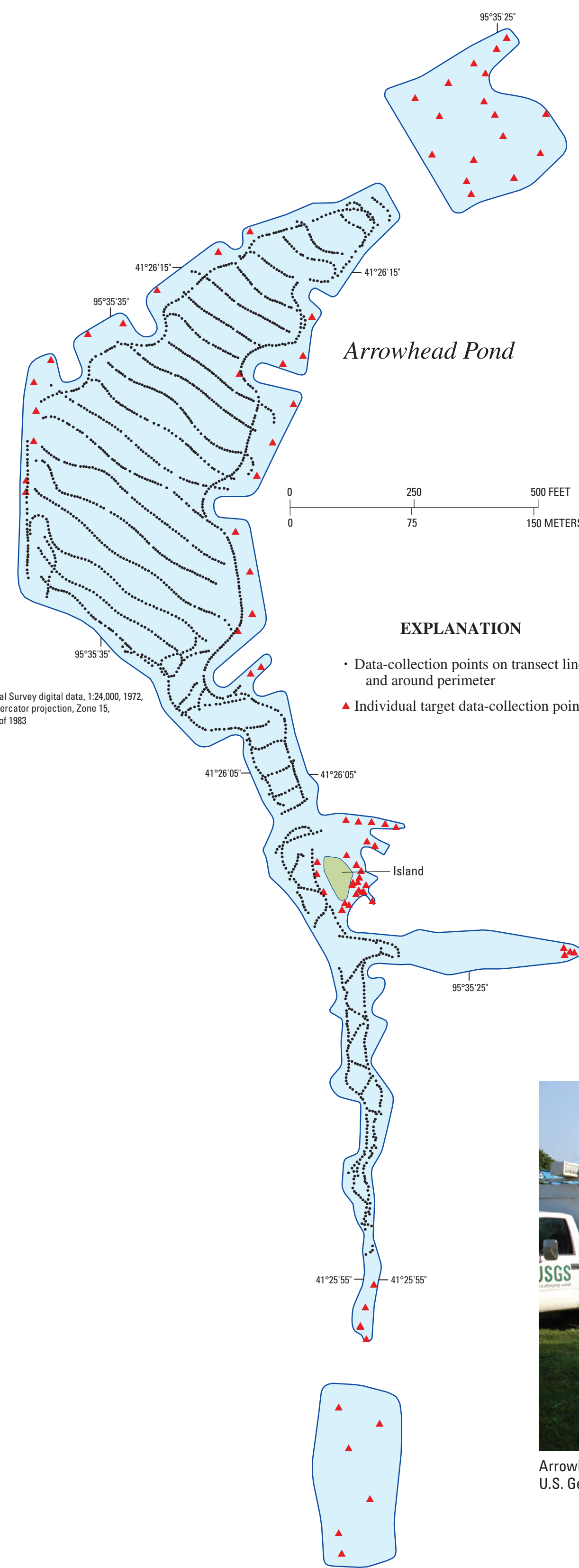
Figure 1. Data-collection points used to construct bathymetric contours.
