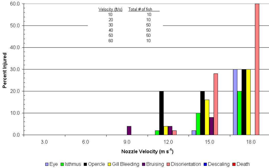
Figure 16. Relative proportions of injury types for all age-0 chinook salmon at each nozzle velocity.
