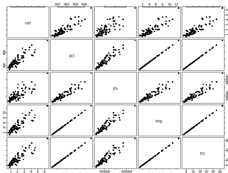
Figure 19. Cross correlation plots derived from the 0.016 s data for each variable examined. Linear plots with no scatter indicate perfect correlations between variables (acceleration, impulse, and force).
