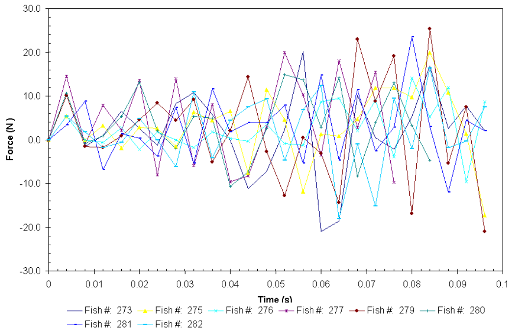
Figure 11. Time series plot of force (mass*acceleration) for a group of the age-1 chinook salmon released at the 15-m·s -1 nozzle velocity.
