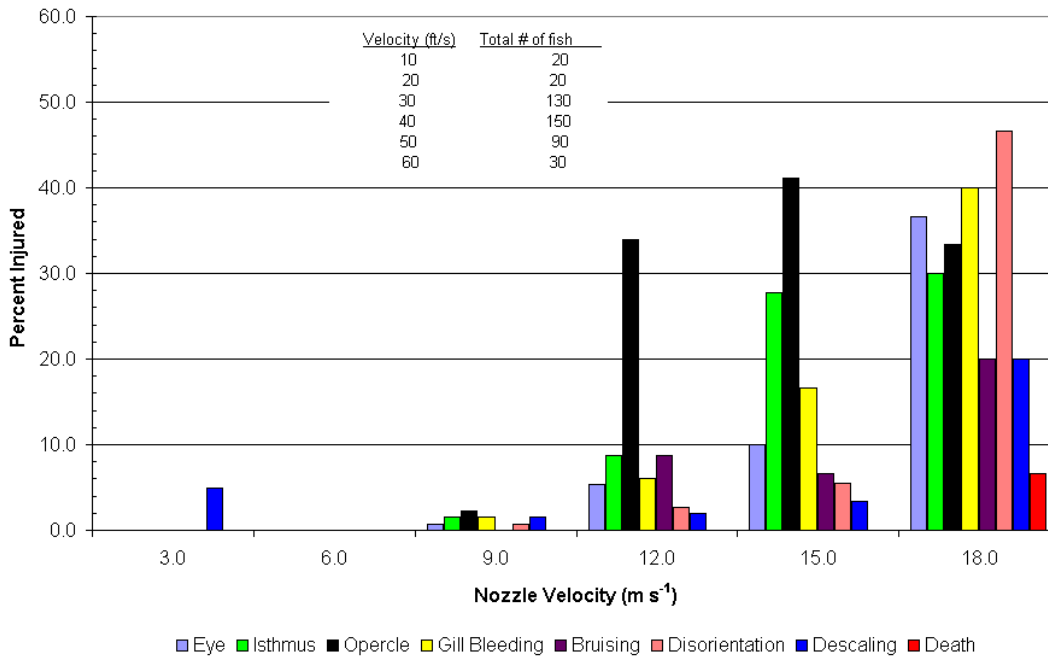
Figure 17. Relative proportions of injury types for all age-1 chinook salmon at each nozzle velocity.
