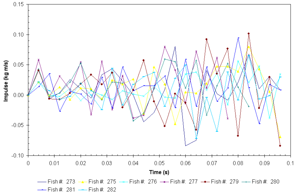
Figure 10. Time series plot of impulse (fish mass*change in velocity) for a group of the age-1 fall chinook salmon released at the 15-m·s -1 nozzle velocity.
