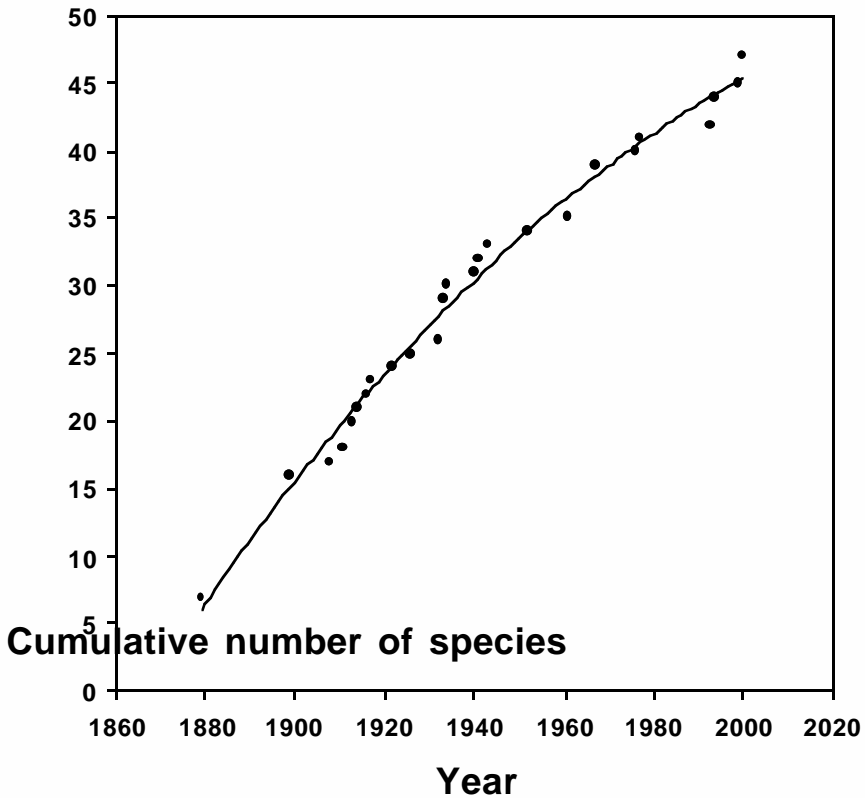
Figure 1. The approximate rate of ant species accumulation in Hawaii. This figure graphs the cumulative number of species documented as established over time, based on the year of first record. Several of these species may no longer occur; see Appendix 1 for information on individual species. The overall trend is fit significantly better by a curve than a line ( F_{1, 23} = 45.628 , P < 0.001 , for comparison of one-term linear model versus two-term quadratic model; R^2 = 0.988 for the fitted curve).
