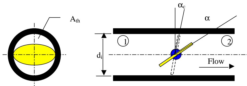
Figure 2.3 Butterfly valve throttle body
