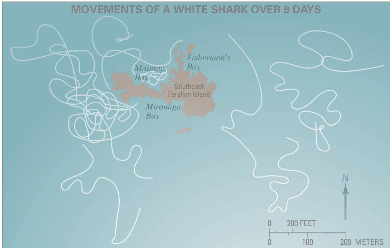
Figure 3. White sharks do not swim aimlessly; they increase their odds of finding seals by looking in familiar areas where they have previously been successful. The map shows the movements of a white shark tracked during October 21–29, 1993, around Southeast Farallon Island, using a transmitter swallowed by the animal.
