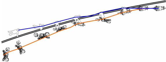
Figure 16. Trajectories of the motorcycle and dummy determined from the overhead view camera before and 230 milliseconds after impacting the modified steel guard rail system (see Figure 15)
