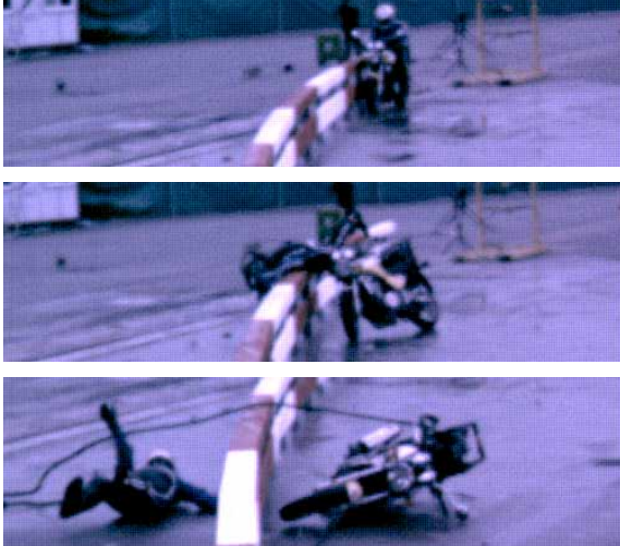
Figure 15. Full-scale crash test where the motorcycle impacts the modified steel guard rail system in an upright position
