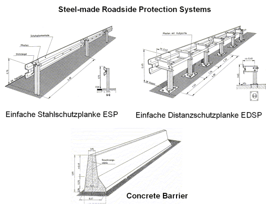
Figure 1. Two steel-guard rails and a concrete barrier common for German roads and investigated with full-scale crash tests
