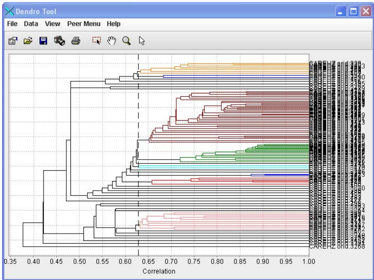
Figure 9. Dendrogram Window
