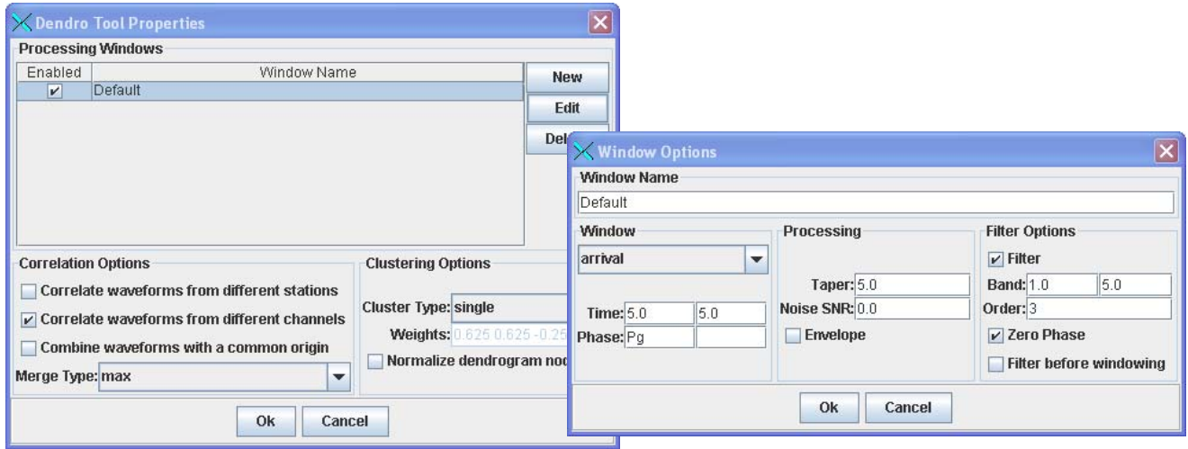
Figure 10. Dendrogram Properties
