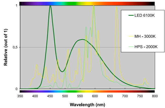
Figure 3. Comparative spectral power distributions for HPS, MH, and LED. Colors shown along top and bottom are approximations provided for reference.
