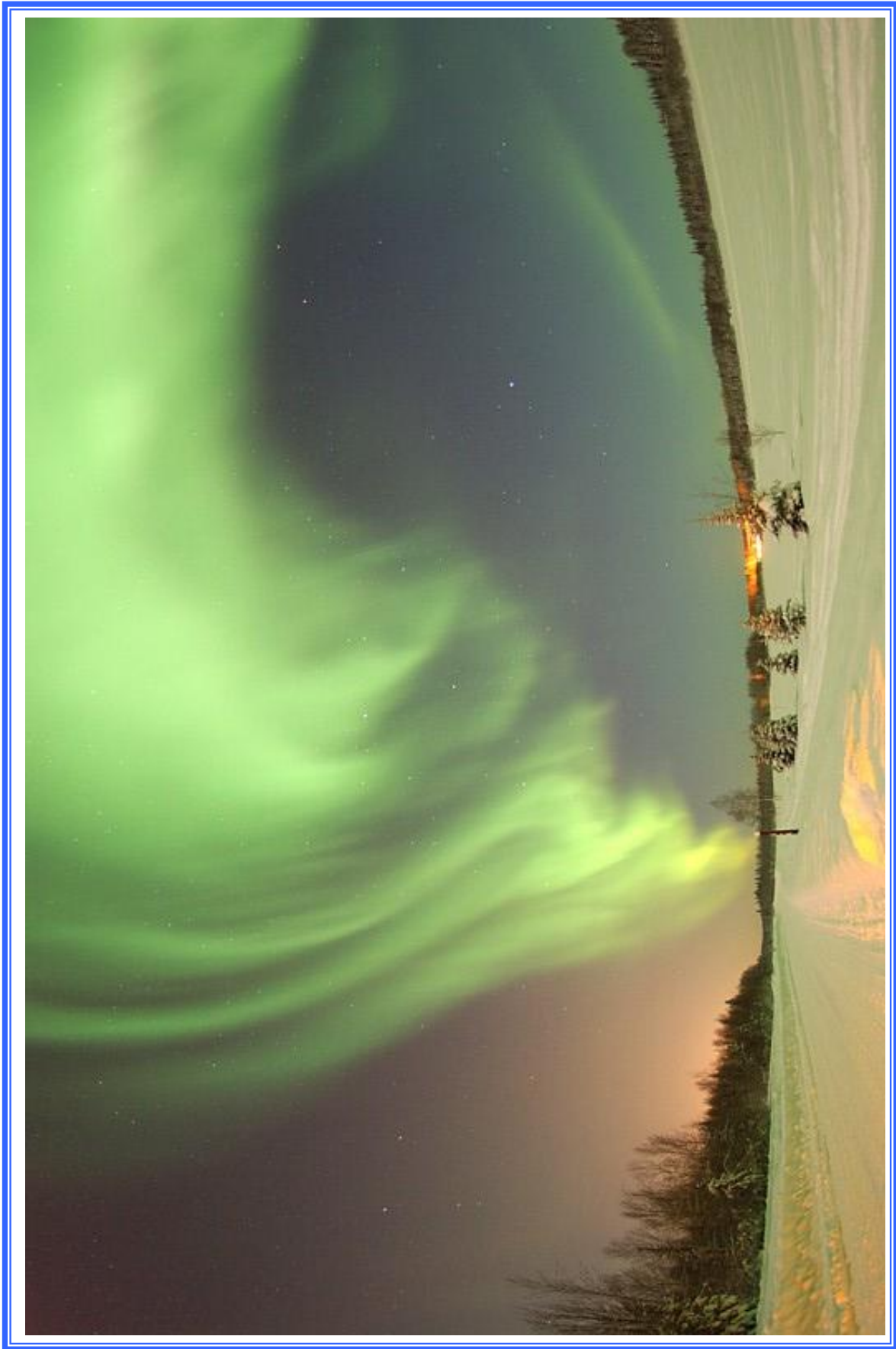
January 18, 2005 aurora photographed above Bear Lake near Eielson Air Force Base, Alaska. Courtesy, The Morrisons http://www.strangecosmos.com/content/item/105349.html
