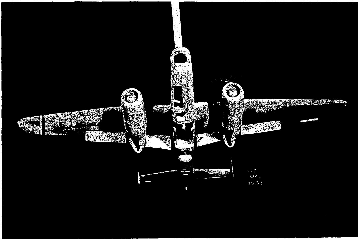
Figure 6.- Photograph of a \frac{1}{11} -size model of the B-25 airplane with simulated damage of wheel and bomb-bay doors, camera and entrance hatches, and bombardier's window.
