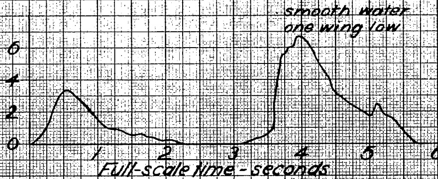
Figure 13. Time history of longitudinal decelerations of a \frac{1}{4} -size model of the Army B-25 airplane, ditched in various conditions of seaway. (Attitude of thrust line, 13^\circ ).
