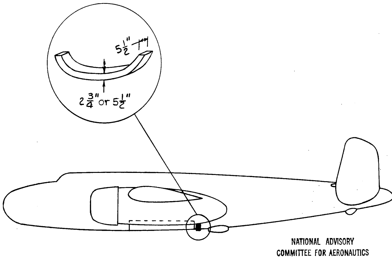
Figure 3. - Projecting ridge as tested on the model of the B-25 airplane. (Dimensions are for the full-size airplane.)
