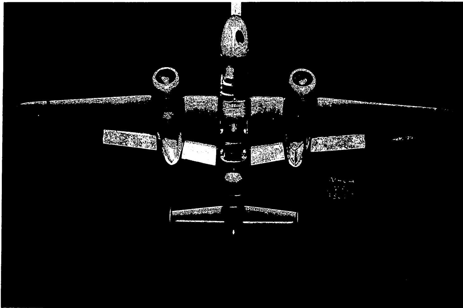
Figure 2a.- Bottom view of a \frac{1}{11} -size model of the B-25G airplane, showing openings cut out to simulate failure of the wheel doors, bomb-bay doors, camera hatch, and bulkhead at the after end of the bomb bay.
