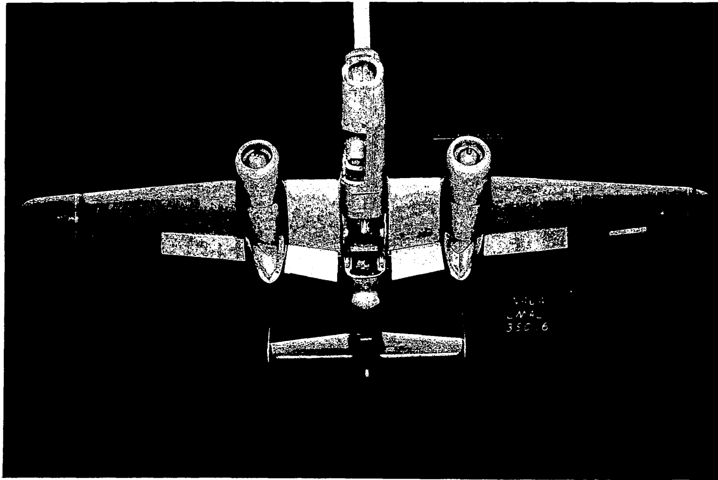
Figure 4.- Photograph of a \frac{1}{11} -size model of the B-25 airplane with simulated damage of wheel and bomb-bay doors, camera hatch, bombardier's window, and the bulkhead at the after end of the bomb bay.
