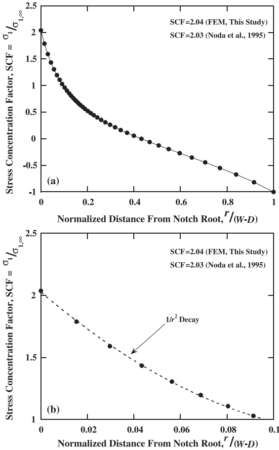
Fig. 4. Stress-concentration effects of the notch in the cantilever beam in the fatigue characterization structure. (a) The normalized stress ( \sigma_1/\sigma_{1,\infty} ) at location, r , along the centerline of the notch is shown as a function of the remaining ligament ( W - D ) of the cantilever-beam structure. The stress concentration factor, SCF, from the finite element model is similar to general results from (Noda and Takase, 1999). (b) The 1/r^2 decay of the maximum principal stress near the root of the notch.
