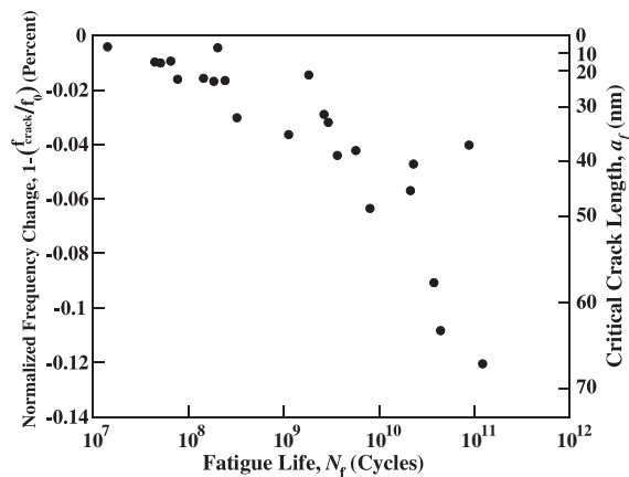
Fig. 12. Decrease in normalized natural frequency, 1 - (f_{\text{crack}}/f_0) , and the associated final crack size, a_f , as a function of specimen life.
