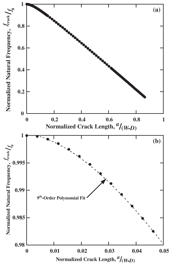
Fig. 5. (a) The relationship between normalized crack length ( a/(W - D) ) and normalized natural frequency ( f_{\text{crack}}/f_0 ) for the plane-stress (full-thickness) finite element model of the notched cantilever beam in the fatigue characterization structure. (b) The behavior for small ( a/(W - D) ) and the associated ninth-order polynomial fit from Table 2 are shown.
