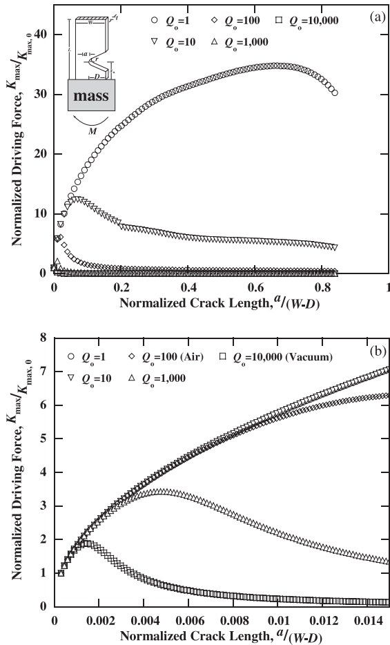
Fig. 9. Stability of a fatigue crack in the resonant-loaded fatigue characterization structure (Fig. 1) predicted by the lumped dynamic model. (a) The normalized driving force for crack advance, K_{\max}/K_{\max,0} , is shown as a function of normalized crack length, a/(W-D) , for the notched cantilever-beam specimen within this structure. Similar to the geometries shown in Fig. 8, the fatigue-crack growth rate will accelerate ( dK/d(a/(W-D)) > 0 ) in heavily damped systems (i.e., low Q_0 ) and will decelerate and possibly arrest ( dK/d(a/(W-D)) < 0 ) if the damping in the system is decreased (i.e., high Q_0 ). (b) Results from the lumped dynamic model for normalized crack lengths relevant to fatigue characterization of polycrystalline silicon ( a/(W-D) < 0.015 ). Fatigue cracks tested in air ( Q_0 \sim 100 ) are always subjected to increasing driving force gradients. However, when the damping is reduced (e.g., Q_0 \sim 10,000 in vacuum) the cracks may arrest due to purely mechanical effects.
