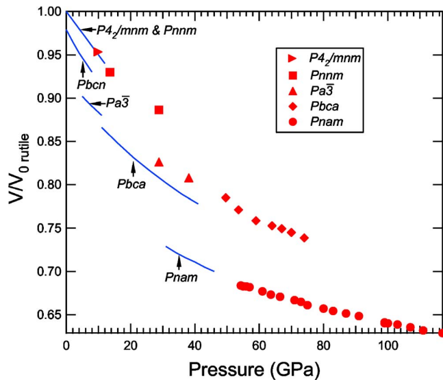
FIG. 6. (Color online) Comparison of compression behavior of \text{PbO}_2 (solid lines) with \text{SnO}_2 (symbols). For each phase, the volume is plotted relative to the zero-pressure volume of the rutile form for that material. Data for \text{PbO}_2 are from Ref. 4, data for \text{SnO}_2 are from this study.
