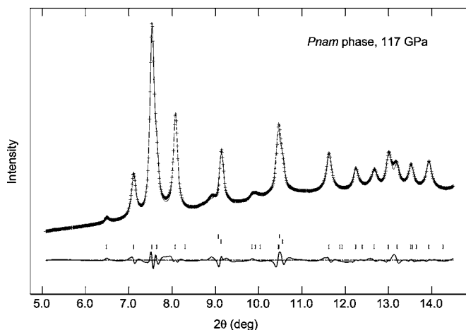
FIG. 5. Rietveld refinement result for Pnam phase. The raw data (crosses) were obtained at 117 GPa, 300 K (after heating). The upper and lower solid lines represent the calculated and the difference curves ( I_{\text{obs}} - I_{\text{calc}} ), respectively. The short vertical bars above the difference curve show reflection positions for each phase (upper: Ar; middle: Pt; lower: Pnam phase). The obtained atomic positions are Sn 4+ [0.2547(18), 0.11422(31), 0.25], O 2- (1): [0.348(4), 0.390(5), 0.25], O 2- (2): [0.043(6), 0.333(4), 0.75], and Rp=1.2 %.
