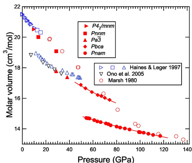
FIG. 4. (Color online) The molar volume as a function of pressure for SnO 2 phases at pressure to 117 GPa. The symbols used here are same as Fig. 2, except for open circles which represent shock compression data from Marsh (Ref. 22). Solid lines are second-order Birch-Murnaghan equation fits to Pbca and Pnam phase data. The Pa3̄ data of Ref. 7 are shown with a down pointing triangle to distinguish them from the results of Ref. 5.
