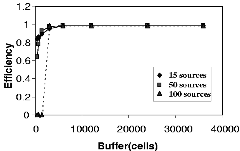
Figure 2: Buffer requirements for single hop LEO
