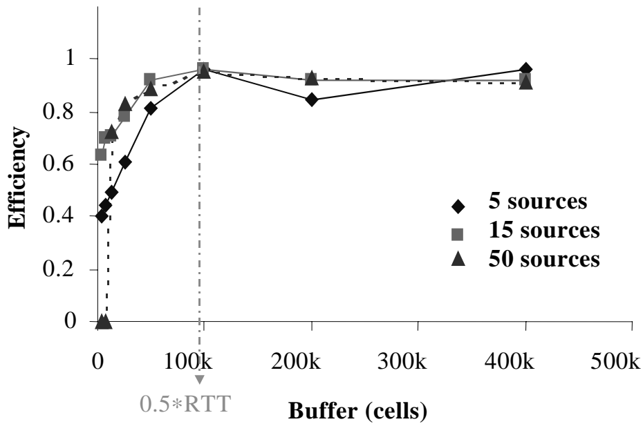
Figure 6: TCP/IP UBR buffer requirements for single hop GEO
