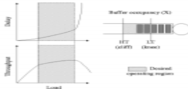
Figure 6: DFBA Target Operating Region
