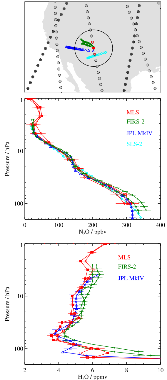
Figure 27. MLS N 2 O and H 2 O ascending orbit overpass measurements (20 September, 2027 UT) compared to the FIRS-2 (20 September, 2034 and 2144 UT), JPL MkIV (21 September, 0043–0147 UT) and SLS-2 (20 September, 1750 UT) measurements from the BOS gondola flown from Fort Sumner on 20–21 September 2005. Horizontal error bars indicate the 1-sigma precisions. Location map details are as in Figure 24 except an additional MLS profile match (red diamond symbol) for N 2 O is shown which matches better the SLS-2 measurement locations.
