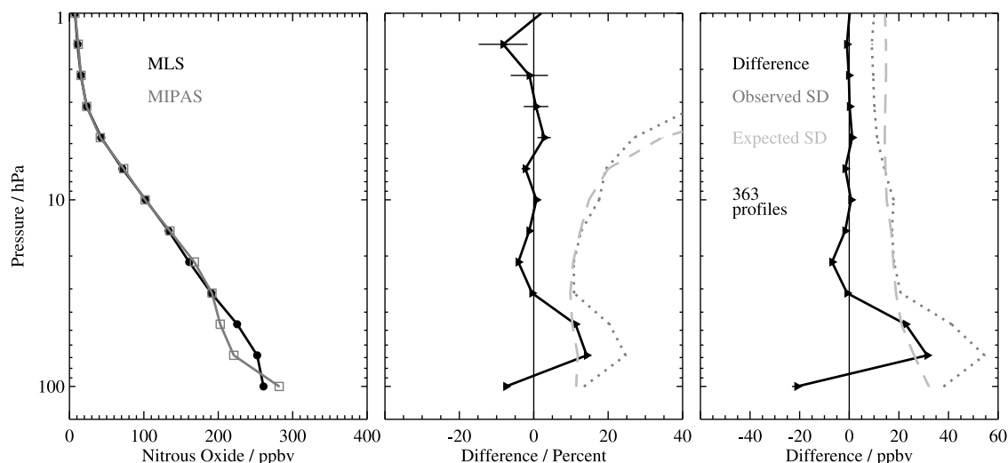
Figure 20. As Figure 13 except for MIPAS N 2 O on 28 January 2005.
