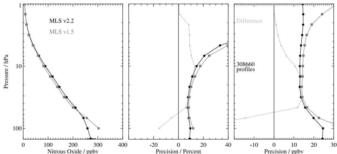
Figure 10. As Figure 9 except for N 2 O.
