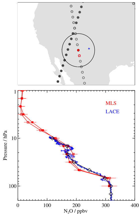
Figure 24. MLS N 2 O ascending orbit overpass measurements (2029 UT) compared to the LACE measurements (1527–2014 UT) from the OMS gondola flow from Fort Sumner on 17 September 2004. The black diamond symbols joined by a solid line indicate the resulting convolution of the high-resolution LACE measurements (blue pluses) with the MLS averaging kernels. The location map shows the MLS overpass ascending (light circles) and descending orbit (dark circles) tangent points. The two closest coincident MLS profiles (see text) are shown as solid (best match) and open red squares. The map scale is indicated by a 500 km radius locus centered on the best match. Horizontal error bars indicate the 1- \sigma precisions. The correlative balloon instrument measurement locations are shown.
