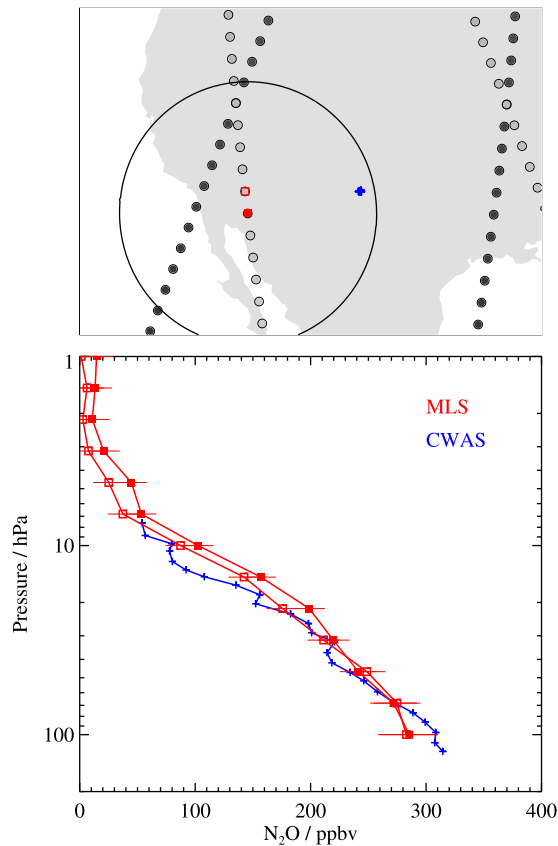
Figure 26. MLS N 2 O ascending orbit overpass measurements (2054 UT) compared to the CWAS measurements (1637–2009 UT) from the OMS gondola flown from Fort Sumner on 29 September 2004. Horizontal error bars indicate the 1-sigma precisions. Location map details are as in Figure 24 except a 1000 km radius locus is centered on the closest matching MLS profile.
