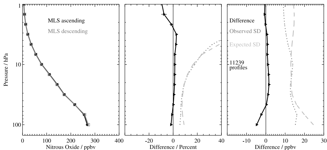
Figure 4. As Figure 3 except for N 2 O.
