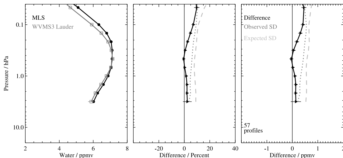
Figure 23. As Figure 13 except for WVMS Lauder H 2 O averaged over 58 d of collocated data. The MLS retrievals have been convolved with the WVMS Lauder averaging kernels.
