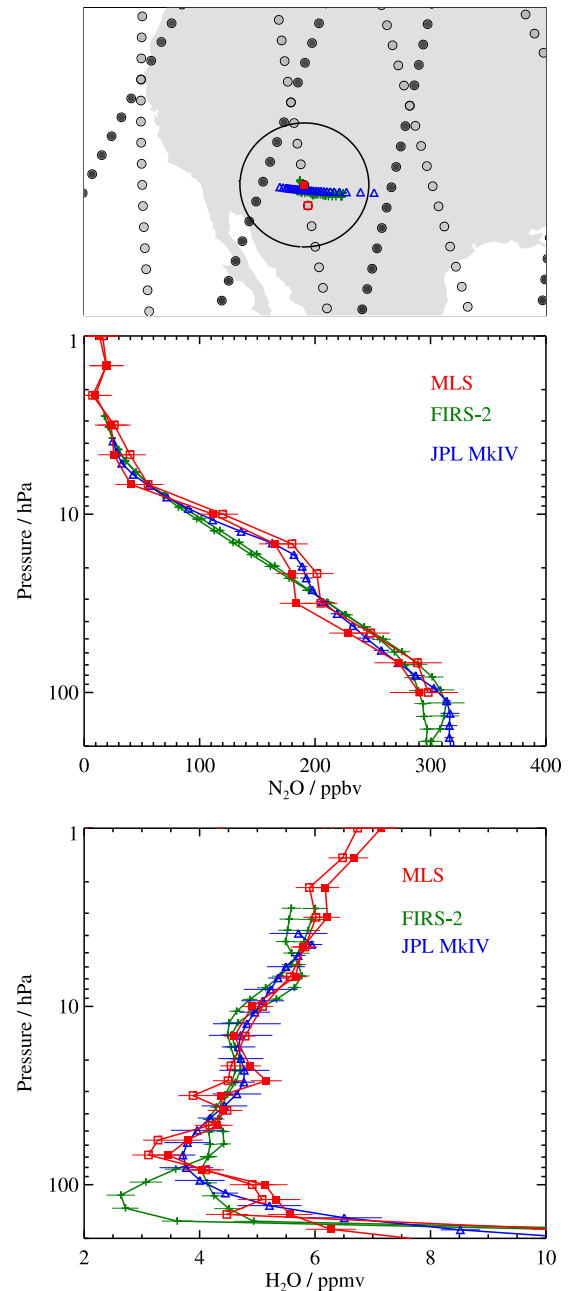
Figure 25. MLS N 2 O and H 2 O ascending orbit overpass measurements (23 September, 2035 UT) compared to the FIRS-2 (24 September, 0233 and 0454 UT) and JPL MkIV (24 September, 0000–0112 UT) measurements from the BOS gondola flow from Fort Sumner on 23–24 September 2004. Horizontal error bars indicate the 1- \sigma precisions. Location map details are as in Figure 24.
