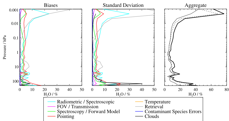
Figure 7. Estimated impact ( 2\text{-}\sigma ) of various families of systematic uncertainty on the MLS H 2 O observations with each family denoted by a different colored line. Cyan lines denote uncertainties in MLS radiometric and spectral calibration. Magenta lines show uncertainties associated with the MLS field of view and antenna transmission efficiency. Red lines depict errors associated with MLS pointing uncertainty. The impacts of uncertainties in spectroscopic databases and forward model approximations are denoted by the green line, while those associated with retrieval formulation are shown in gray. The gold lines indicate uncertainty resulting from errors in the MLS temperature product, while the blue lines show the impact of similar “knock on” errors in other species. Cloud impacts are shown as the thin black line. (left) Estimated bias. (middle) Standard deviation about the bias. (right) Root sum square of all the possible biases (thin solid line), all the additional scatter (thin dotted line), and the RSS sum of the two (thick solid line).
