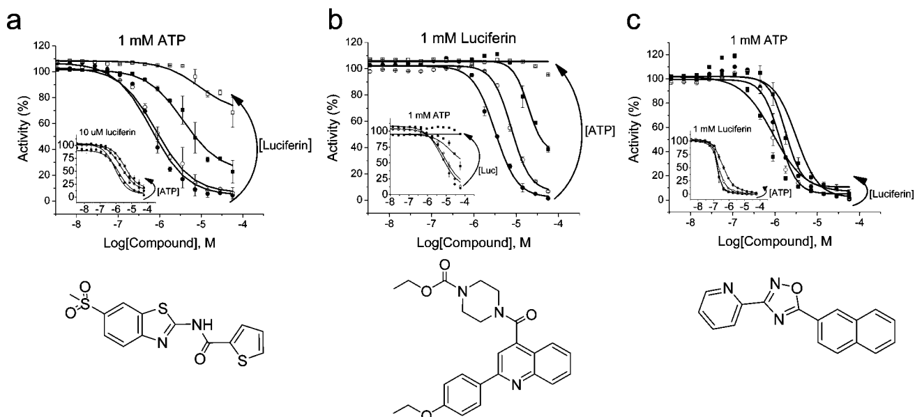
Figure 5. Dependence of inhibition on substrate concentration for three representative series. Luciferin or ATP was varied at (●) 1 \mu M, (○) 10 \mu M, (■) 100 \mu M, and (□) 1000 \mu M. (a) Substrate variation data for the benzothiazole ( 1a ). The graph shows that inhibition can be relieved upon increasing the luciferin concentration, and the inset graph shows that ATP variation has little effect on the inhibition (holding the luciferin concentration constant at 10 \mu M, approximately the K_m ). (b) Substrate variation data for the quinoline ( 4e ). The graph shows that inhibition can be relieved when either the ATP or the luciferin concentration (inset graph) is increased. (c) Substrate variation data for the 1,2,4-oxadiazole ( 5c ). The graph shows that the inhibition remains relatively constant when varying either the luciferin or the ATP concentration (inset graph).
