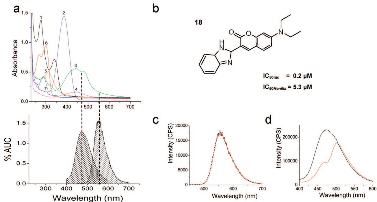
Figure 7. Evaluation of light attenuation by luciferase inhibitors. (a) Top absorbance spectra are shown for quinolione 4a (1, black), ( Z )-( R 1 amino)prop-2-en-1-one 6a (2, purple), coumarin 20 (3, green), mGluR5 antagonist 16 (4, magenta), benzthiazole 1d (5, orange), benzamide 7a (6, red), and oxadiazole 5c (7, blue). Lower graph on left shows the luminescence spectra of R. reniformis luciferase (left spectrum) vs firefly luciferase (right spectrum). Emission spectra are shown as percentages of the AUC for each spectrum. Dotted lines correspond to the emission maxima. (b) Structure of coumarin 18 and potencies for firefly and R. reniformis luciferases. (c) Firefly luminescence in the absence (black line) and presence (red line) of 100 \mu M compound 18 . (d) R. reniformis luminescence in the absence (black line) and presence (red line) of 100 \mu M compound 18 .
