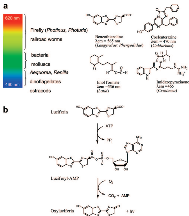
Figure 1. Bioluminescence of the luciferin–luciferase reaction. (a) The spectrum of bioluminescence is shown at left along with the names of the organisms that produce the luminescence. Also shown at right are luciferins for firefly ( Lampryidae ) and railroad worms ( Phengodidae ), sea pansies and jellyfish ( Cnidarians ), mollusks ( Latia ), and ostracods ( Crustacea ; the ostracod Cypridina ( Vargula ) hirgendorffii ). (b) Enzymatic reaction of Photinus luciferase. Luciferin and adenosine 5'-triphosphate (ATP) substrates are used by luciferase to form a luciferyl–adenosine 5'-monophosphate (AMP) intermediate that is subsequently oxidized in the presence of oxygen to generate light, as well as the products oxyluciferin, CO 2 , and AMP.
