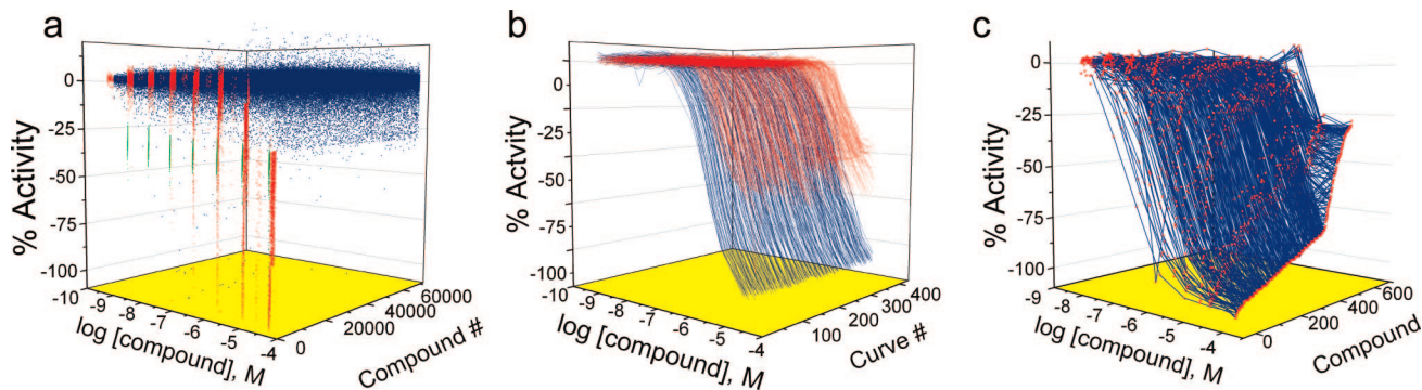
Figure 2. Luciferase qHTS. (a) Concentration–response data are shown for active (red) and inactive (blue) compounds. Activities for 352 compounds (green) were reduced because of a partially occluded reagent dispenser tip. (b) Titration–response curves for the control luciferase inhibitors, resveratrol (blue) and apigenin (red). (c) Representation of class 1 concentration–response curves derived from the qHTS. Data points are shown in red with blue wire-frames drawn through the points to represent the concentration–response curves.
