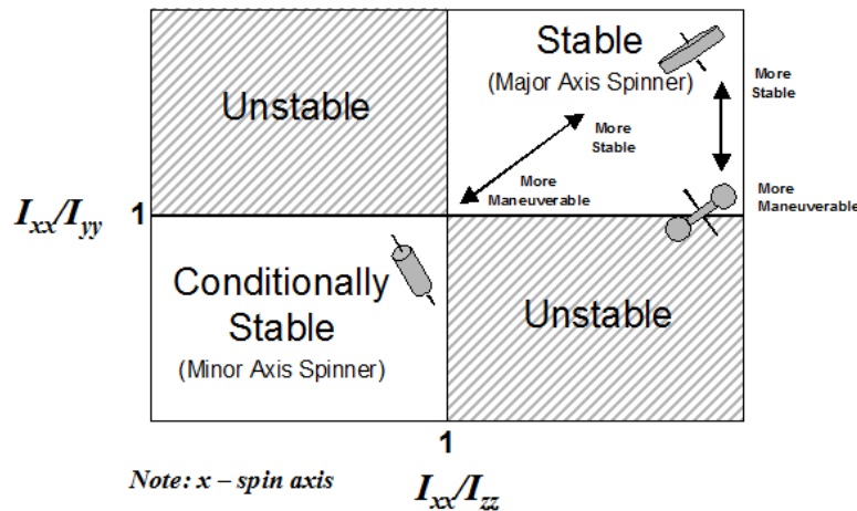
Figure 6. Rotational Stability
