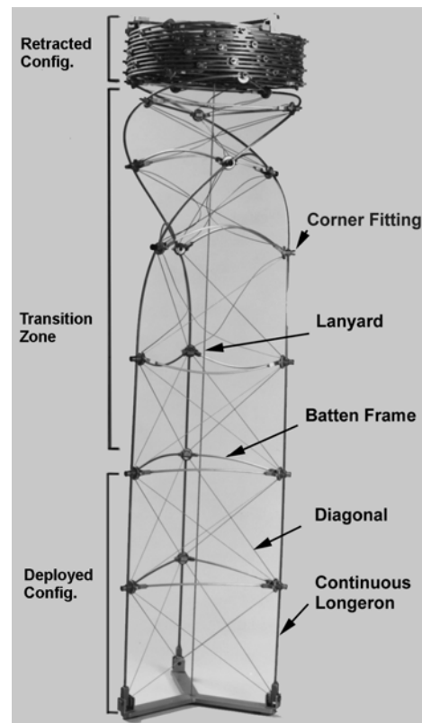
Figure 10. Coilable Mast Concept
