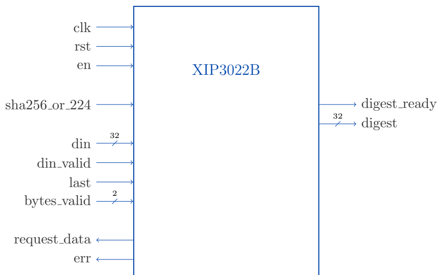
Figure 2: External interfaces of XIP3022B
