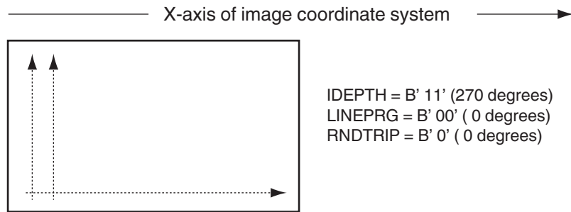
Figure 17. IDE Progression
