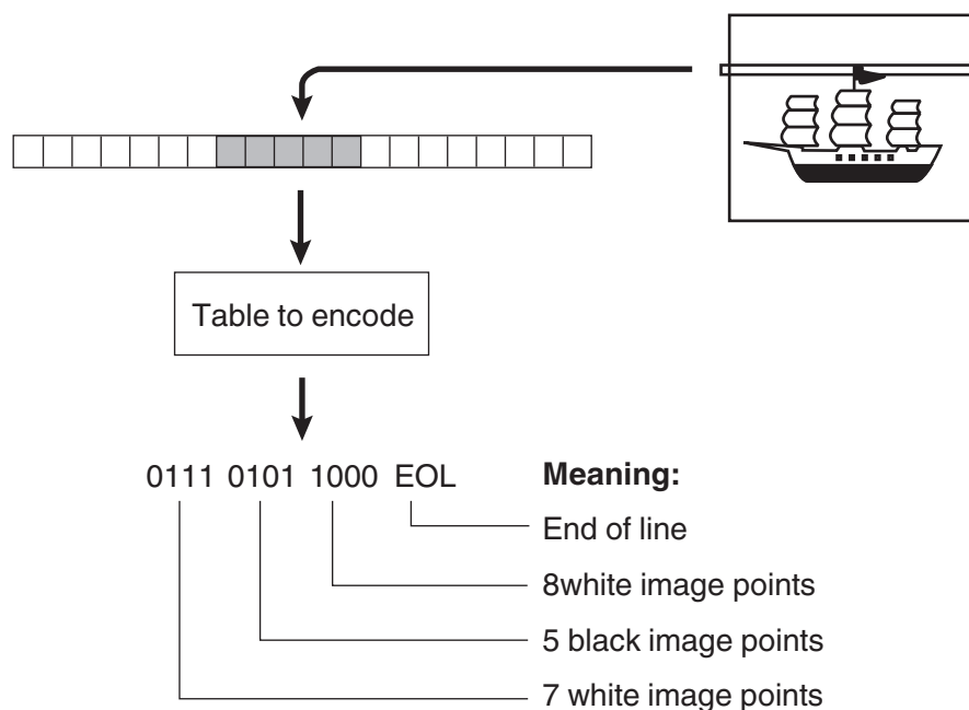
Figure 10. Image Compression
