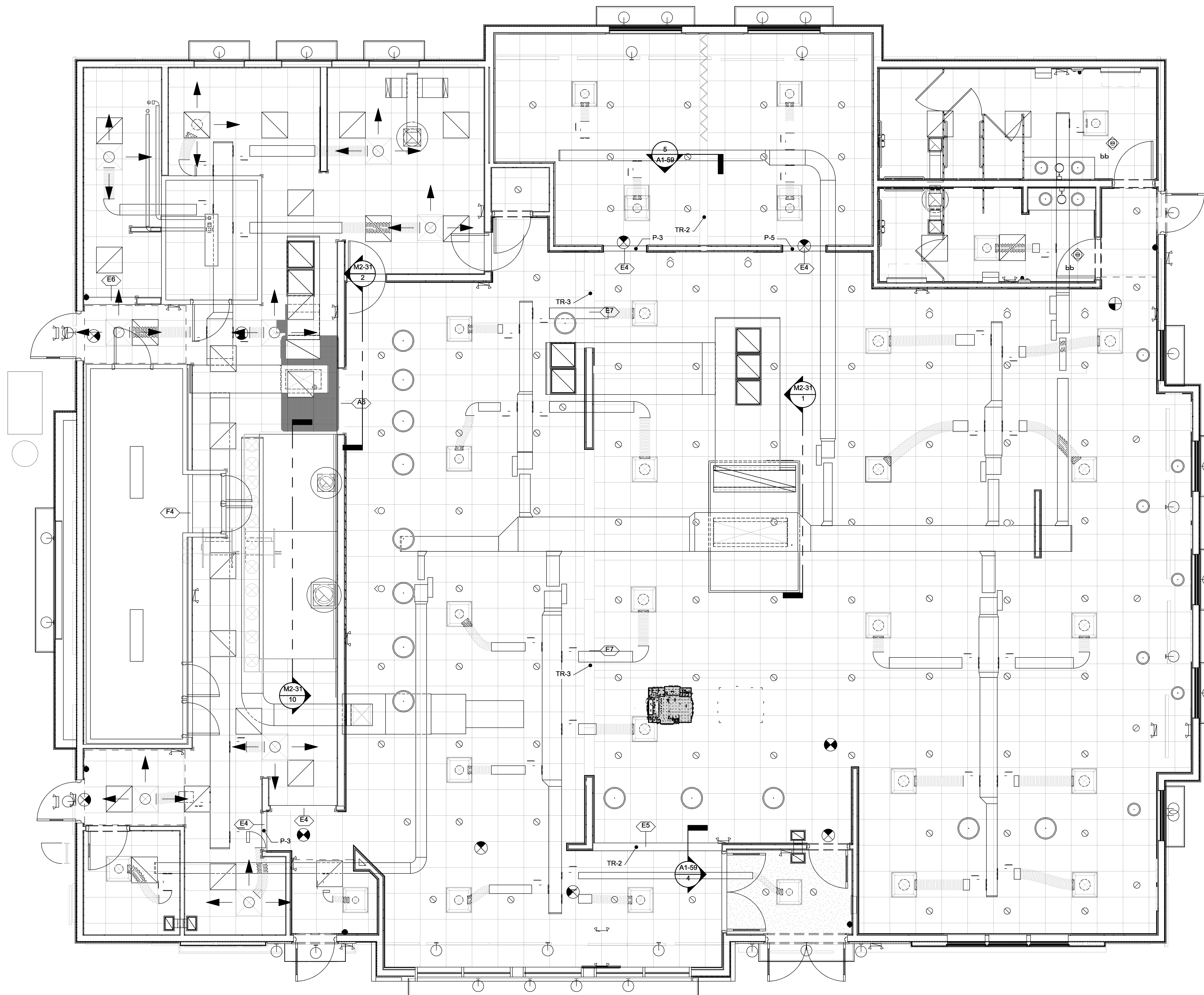
1 MECHANICAL AND LIGHTING COORDINATION CEILING PLAN - FOR REFERENCE ONLY 1/4" = 1'-0"
