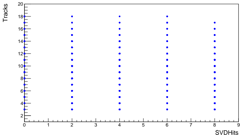
nTracks:pi_nSVDHits
