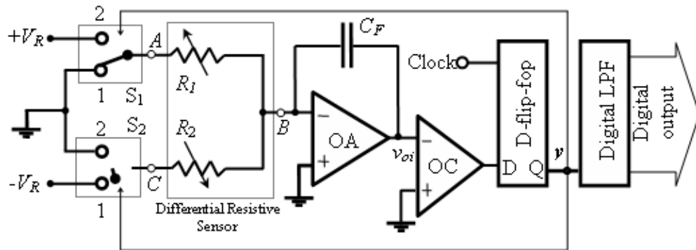
Fig. 2 Proposed sigma-delta resistance to digital converter
