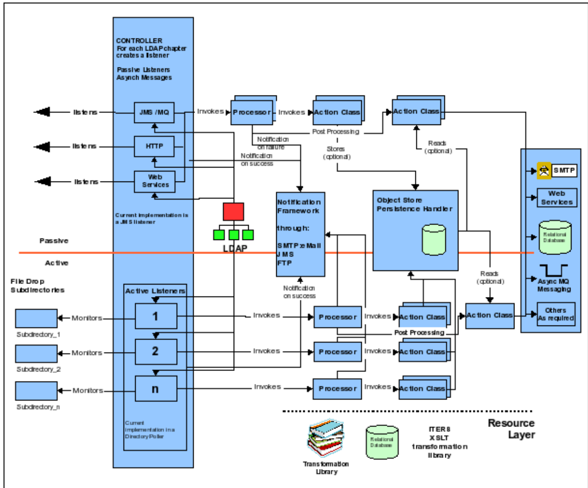
Figure 2.2. Example JBoss SOA Platform deployment
