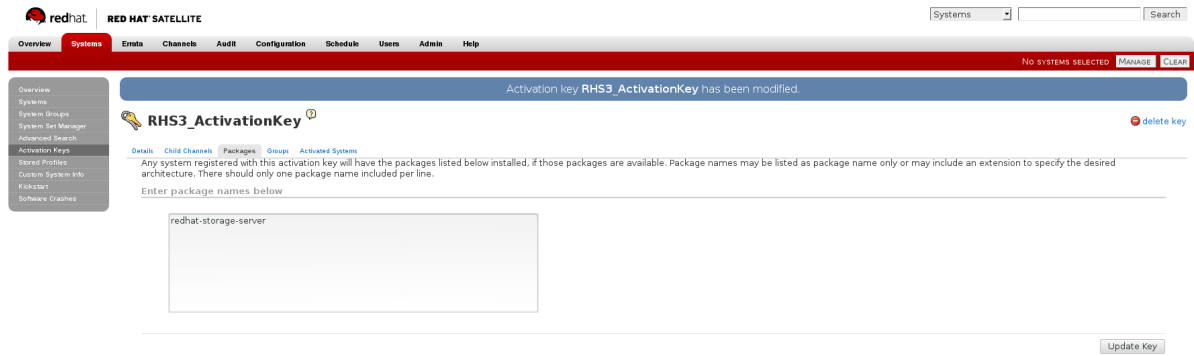
Figure 2.6. Package
