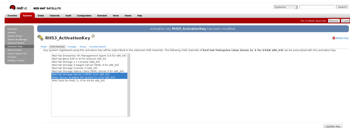
Figure 2.5. Child Channels
