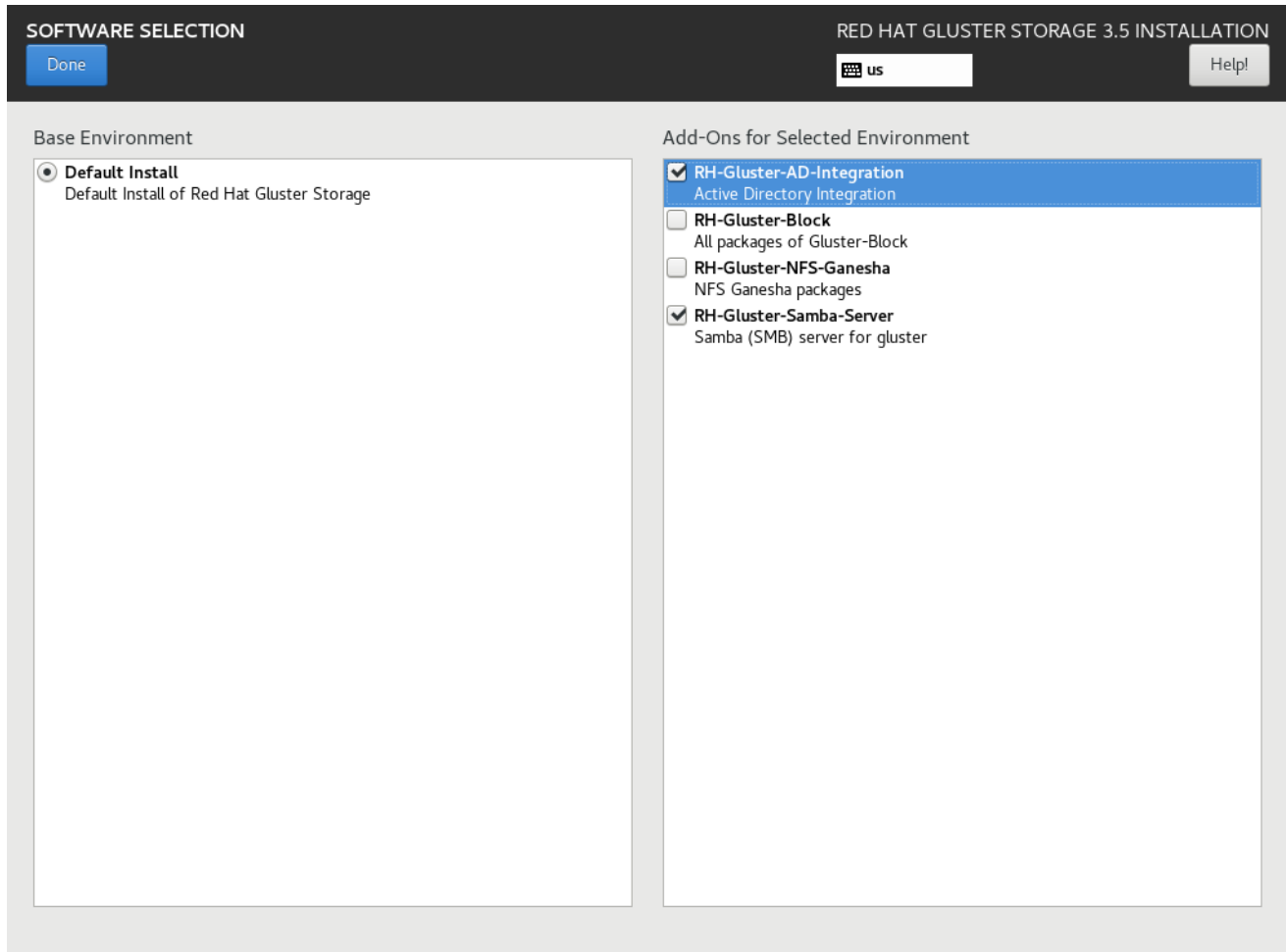
Figure 3.1. Customize Packages
