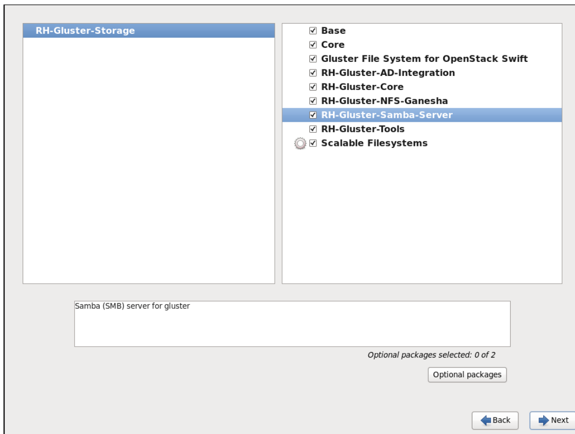
Figure 2.2. Customize Packages
