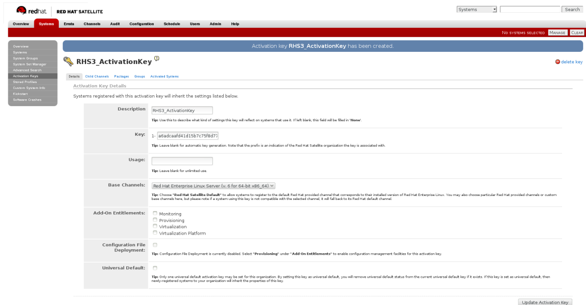
Figure 2.4. Base Channels
