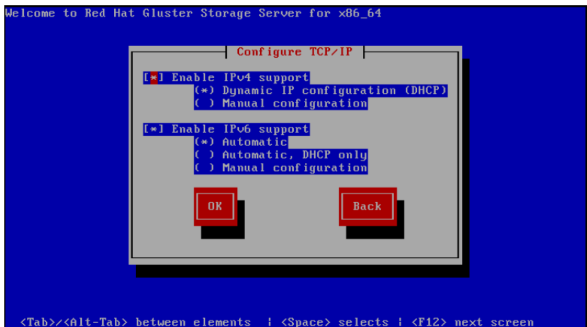
Figure 2.1. Configure TCP/IP
