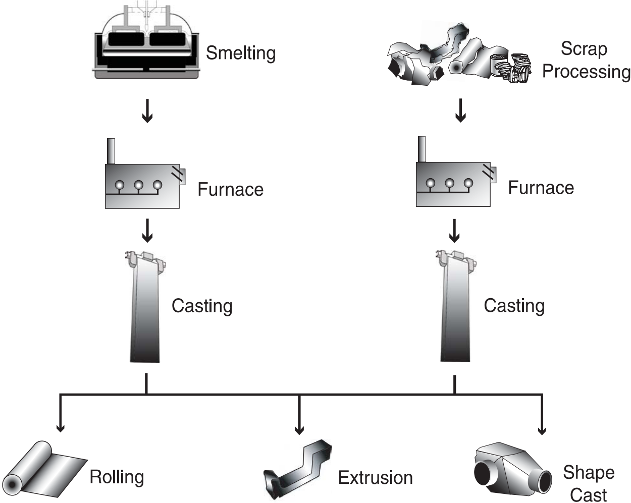
Diagram A - Aluminum Industry Flow Diagram
