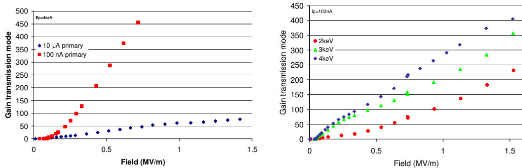
FIGURE 9&10. Left: TM gain of single crystal CVD diamond vs. field in diamond for 4keV primary energy at 293K with 100nA and 10μA primary current. Right: TM gain of single crystal CVD diamond vs. field in diamond for primary energies of 2-4keV at 81K with 100nA primary current.
