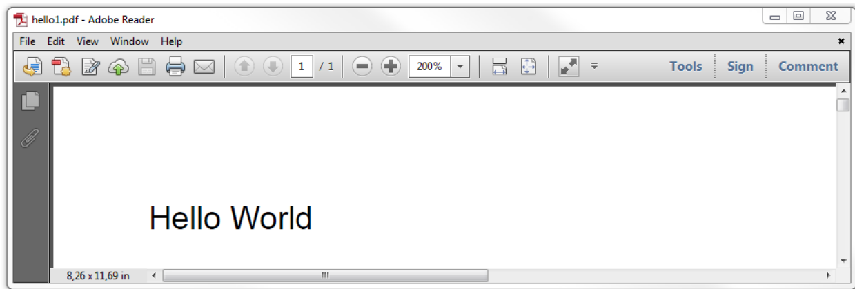
Figure 2.1: Hello World
