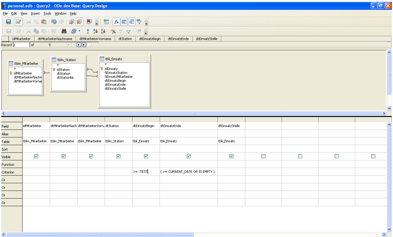
Illustration 1: Start query
