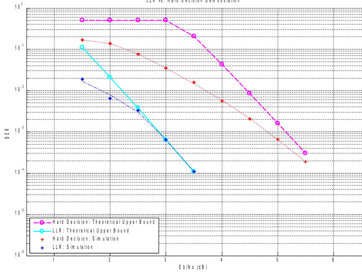
LLR vs. Hard Decision Demodulation
