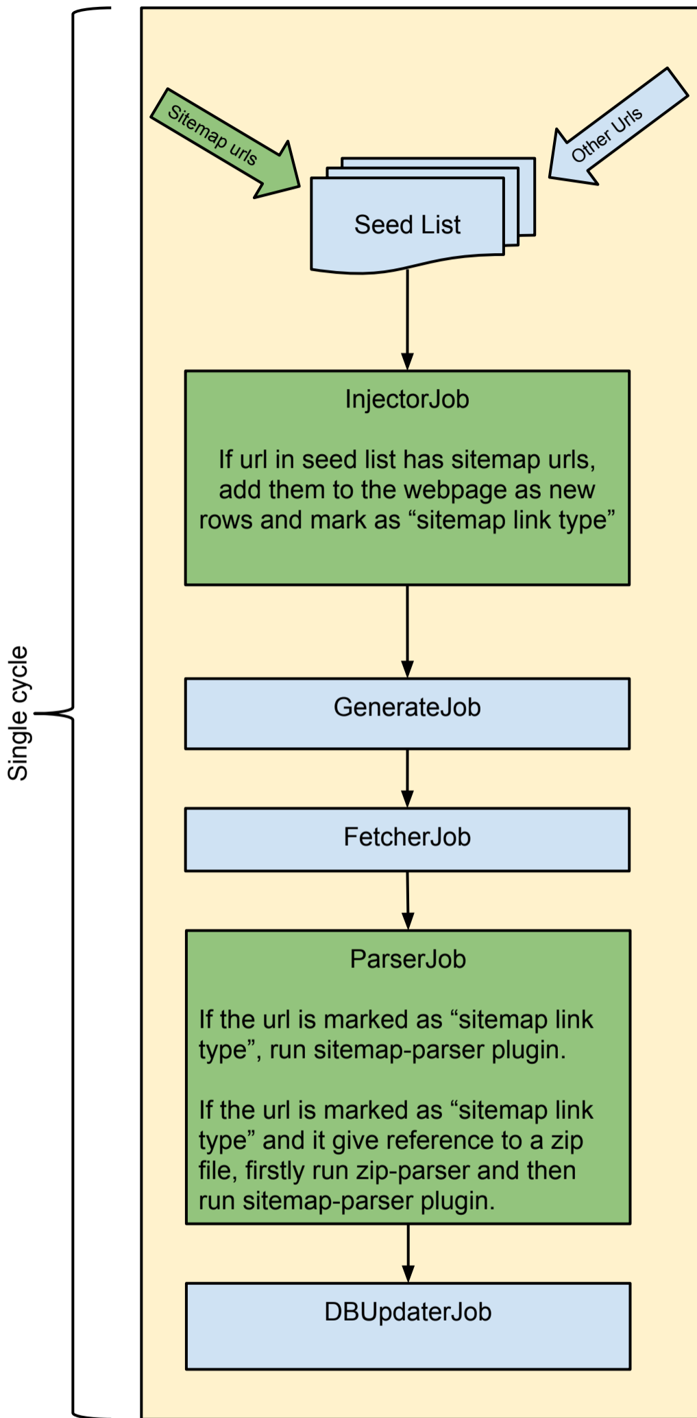
Diagram 1 -Sitemap urls Injection via seedlist
