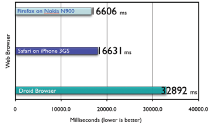
SunSpider JavaScript Benchmark, Dec 2009
