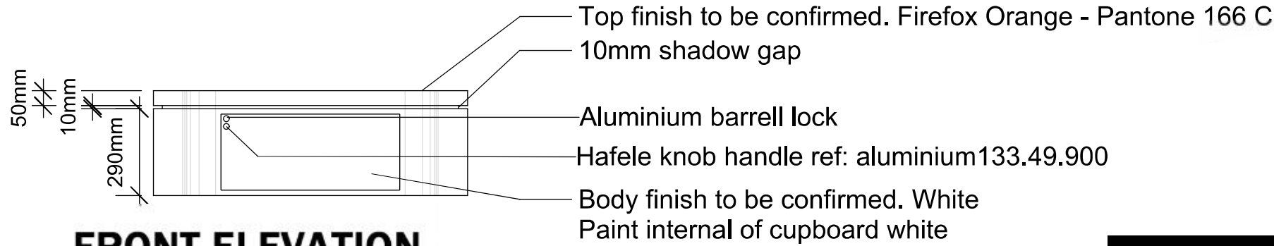
FRONT ELEVATION
