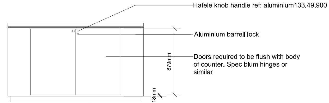
REAR ELEVATION
