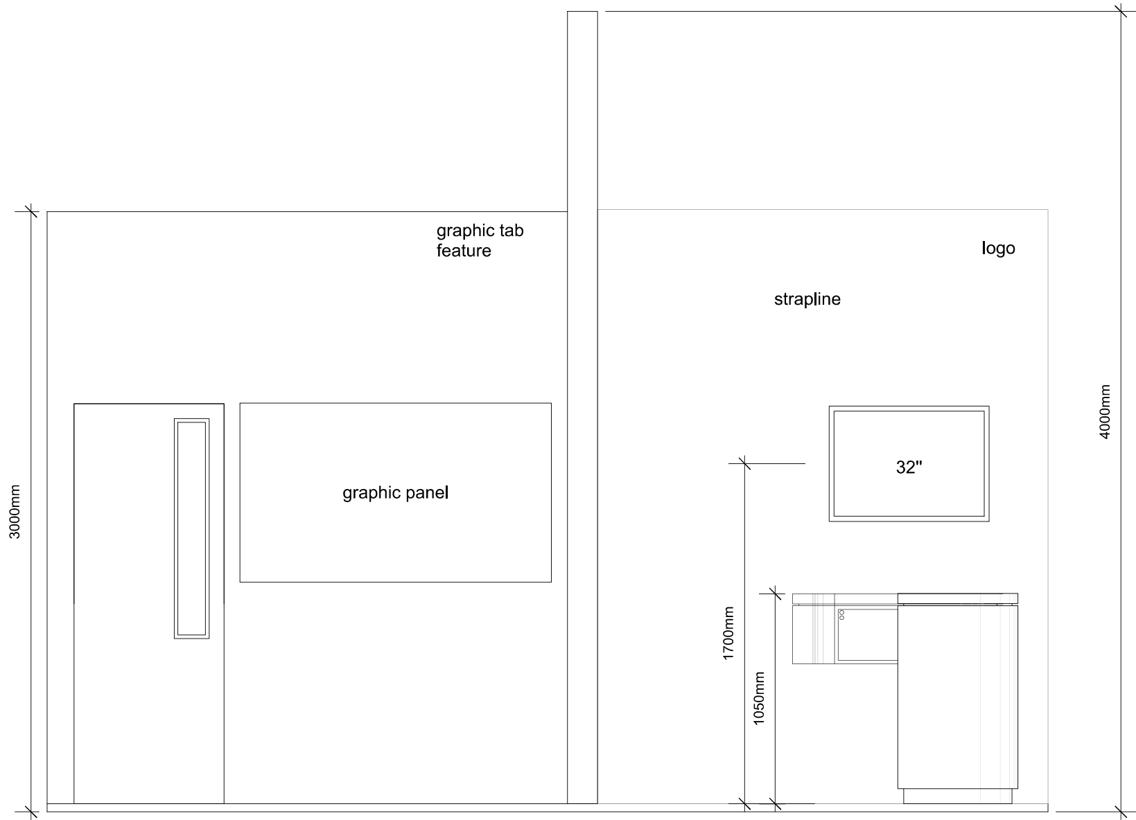
SIDE ELEVATION
