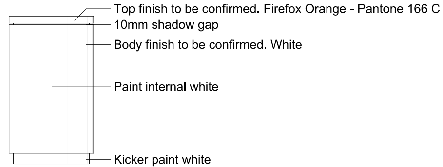
SIDE ELEVATION
