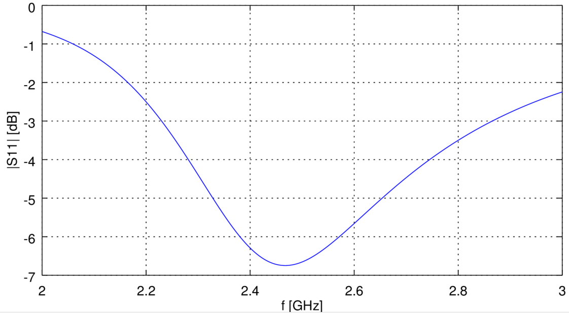
Return loss of flat antenna
