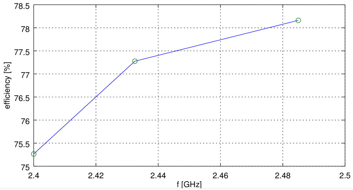
Total efficiency of flat antenna
