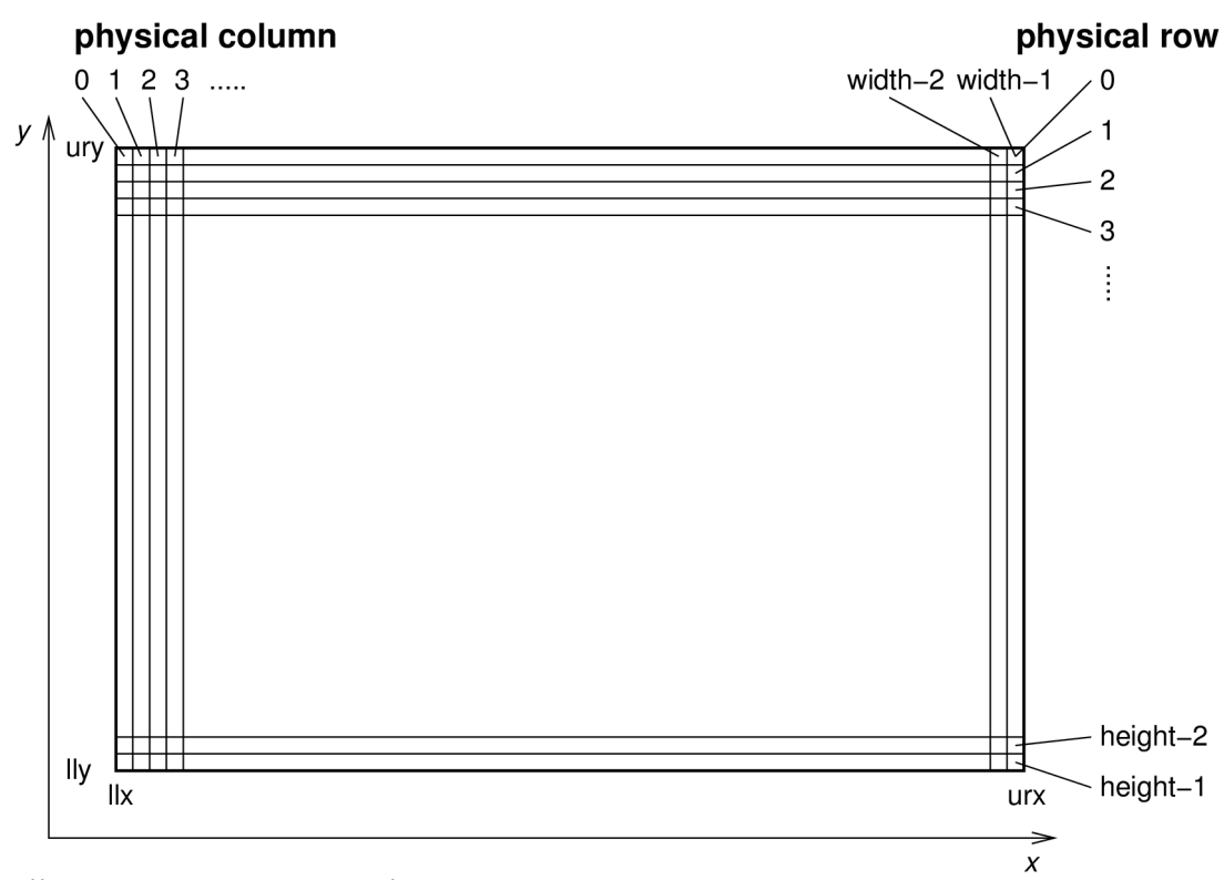
Illustration 1: HPGS scanlines
