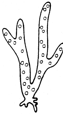
⑥ siphonal
