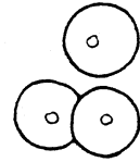
④ coccal
