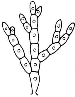
⑤ trichal
