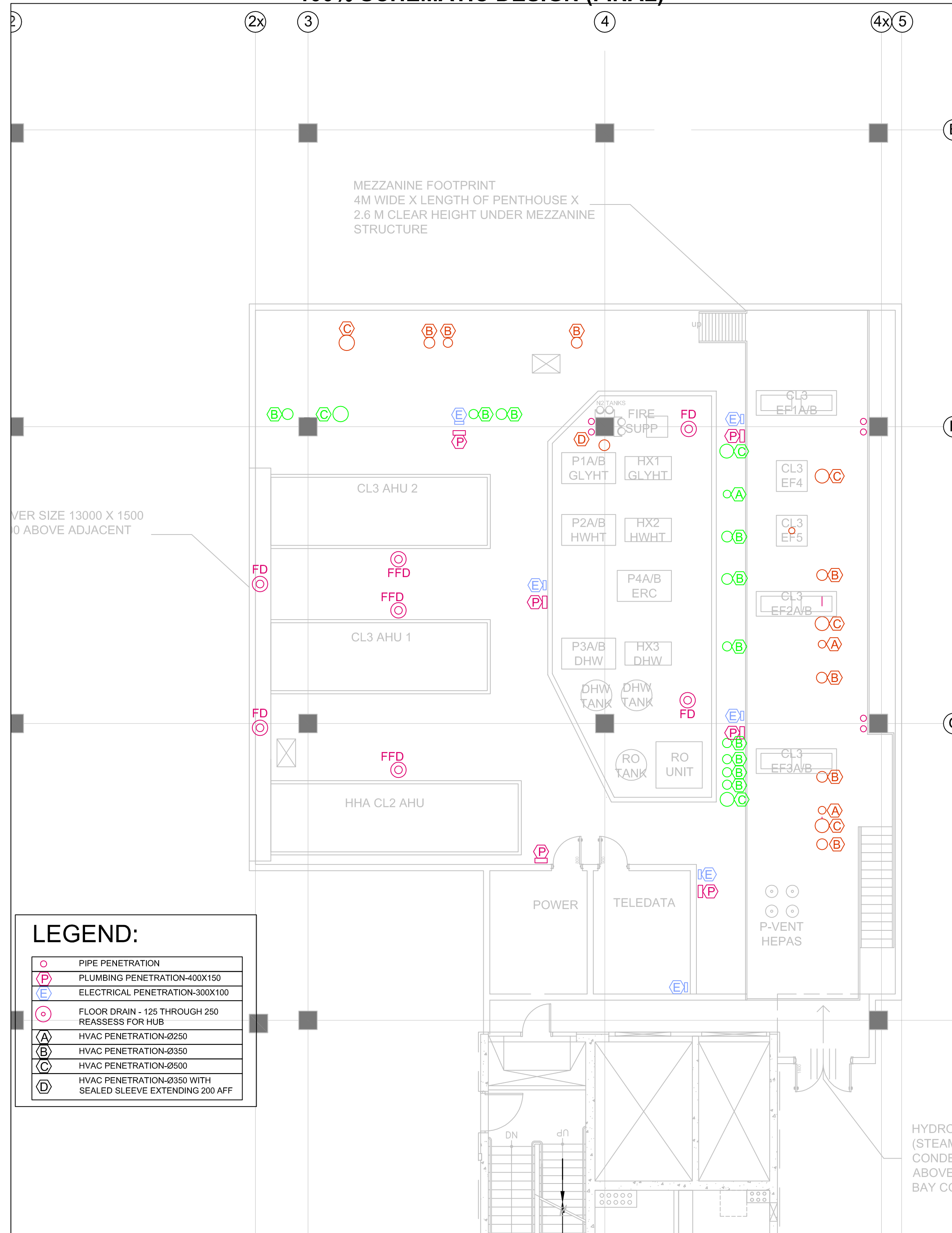
PENTHOUSE SLAB PENETRATIONS SCALE 1:100
