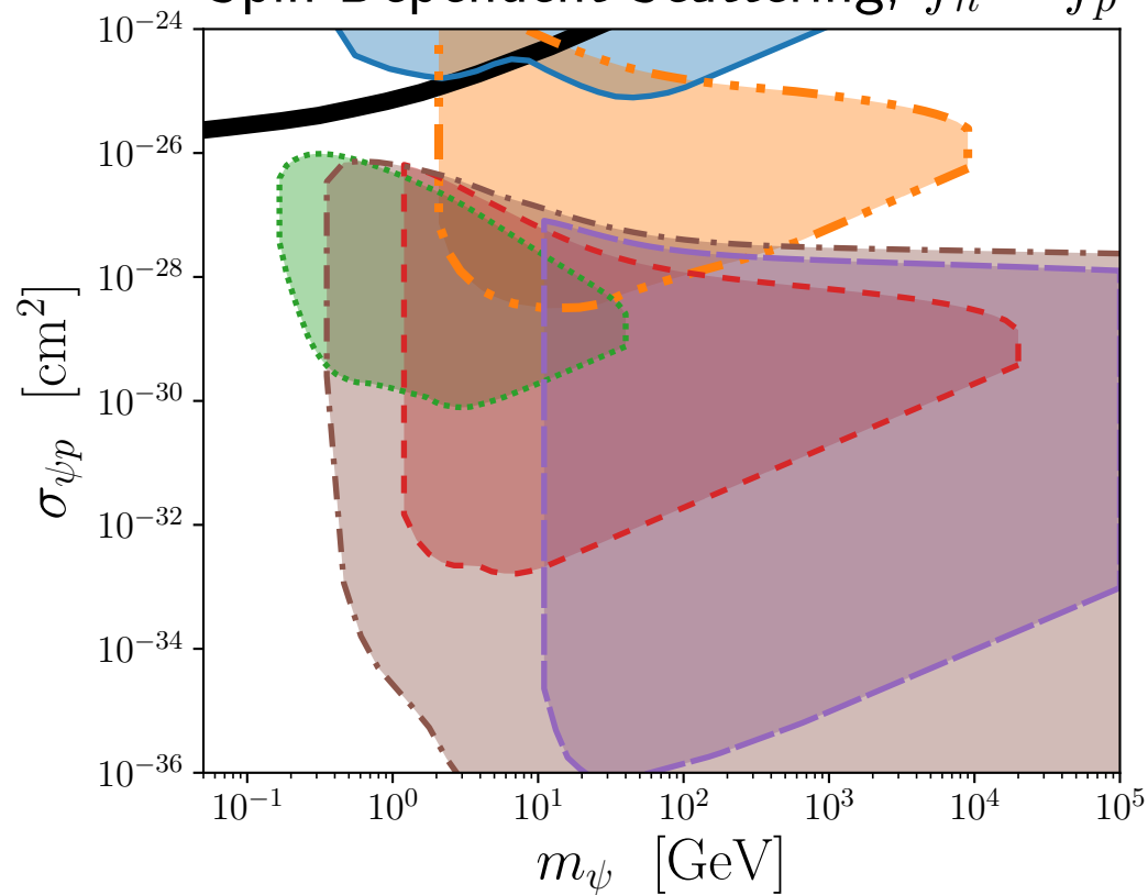
Spin-Dependent Scattering, f_n = f_p
