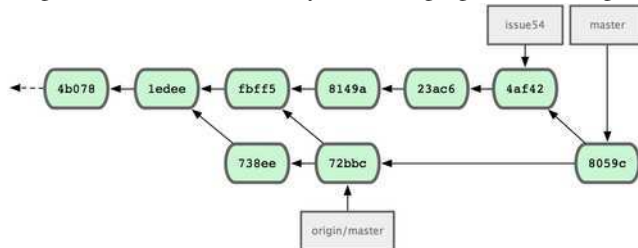
Figure 5.9: Jessica's history after merging John's changes
