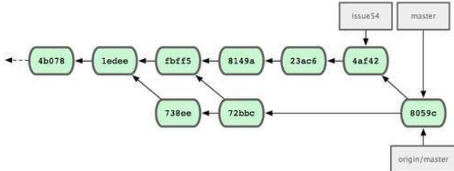
Figure 5.10: Jessica's history after pushing all changes back to the server
