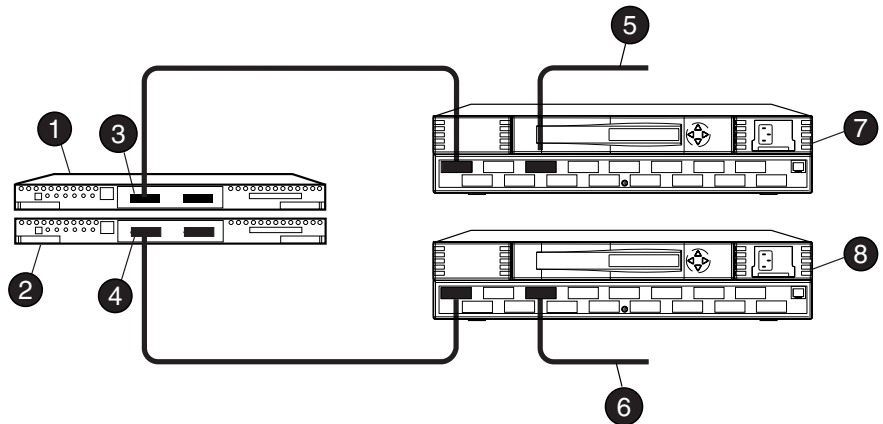
Figure 3-2. Cabling Two RAID Controllers and Two SAN Switches
