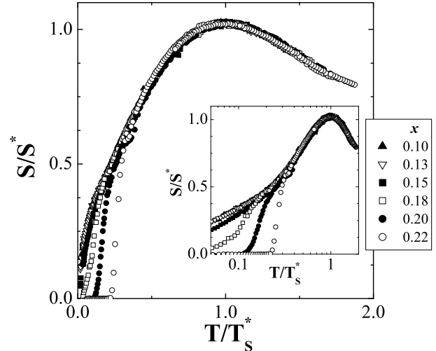
FIG. 3: S/S^* as a function of T/T_S^* for different Ca contents of the double-layer Y_{1-x}Ca_xBa_2Cu_3O_6 . The inset shows S/S^* vs T/T_S^* on the logarithmic scale.
