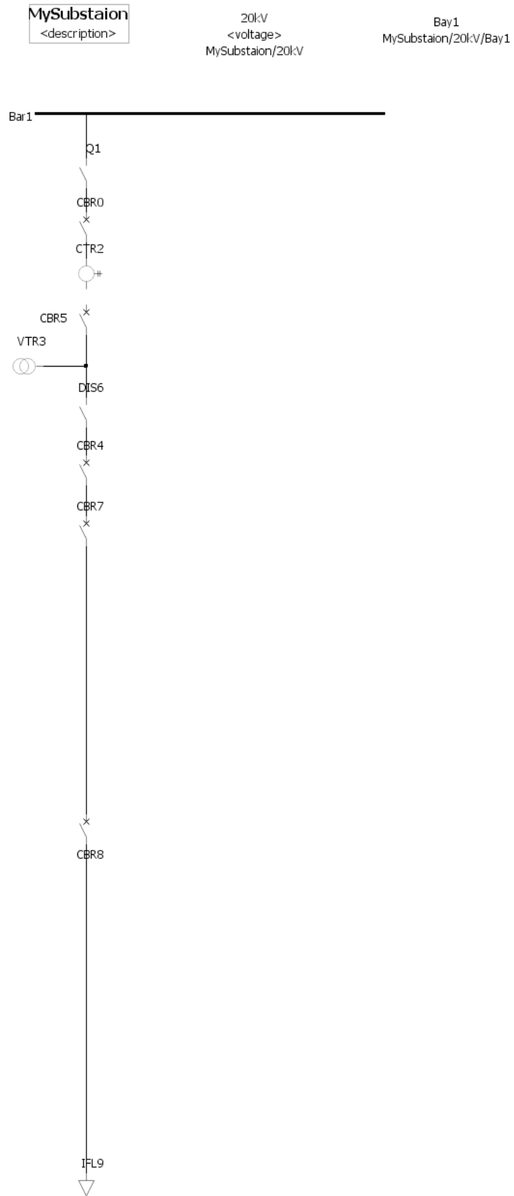
Figure 1. System Diagram of MySubstaion
